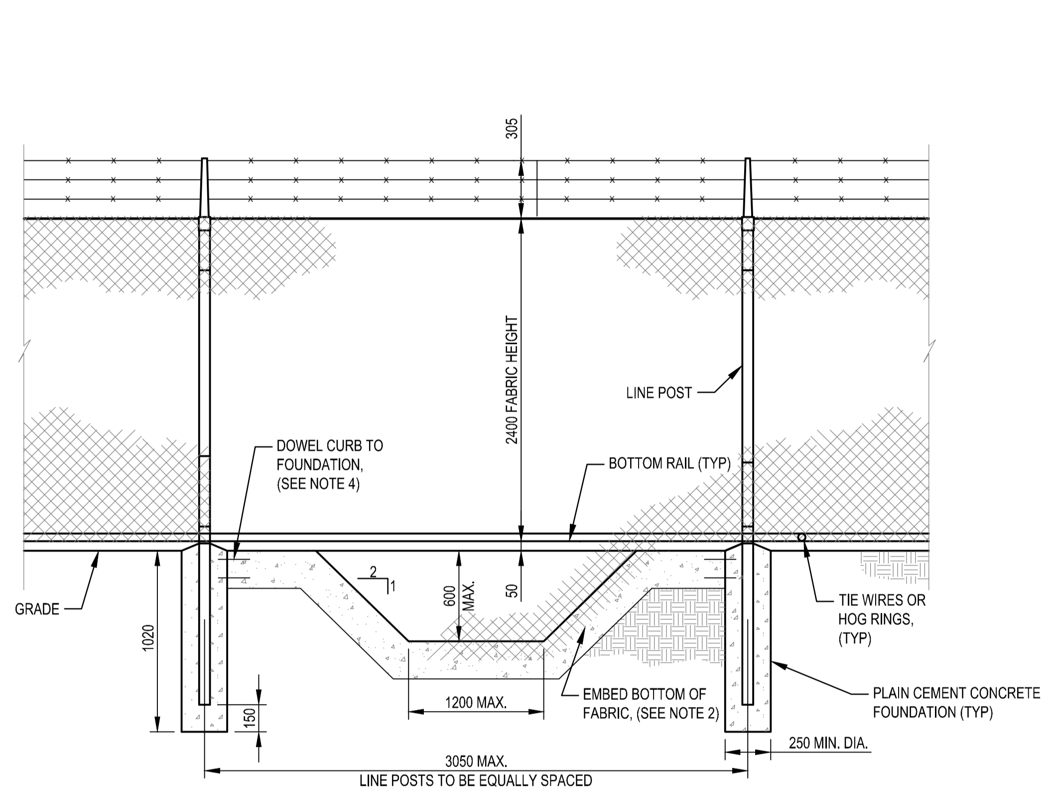
1 DETAIL - SWALE CROSSING SCALE: NTS
